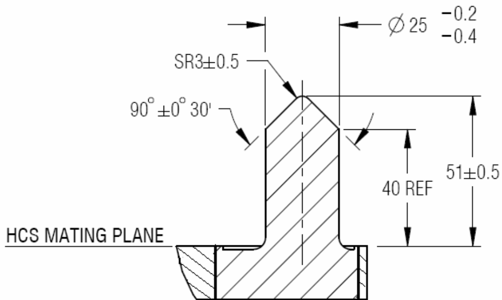
Figure 3-12b: Section C-C
