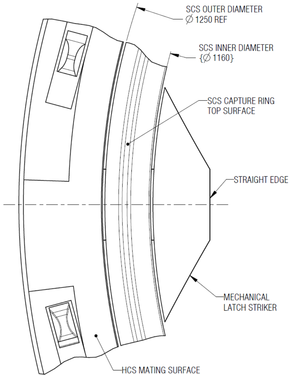
Figure 3-8c: Top View
