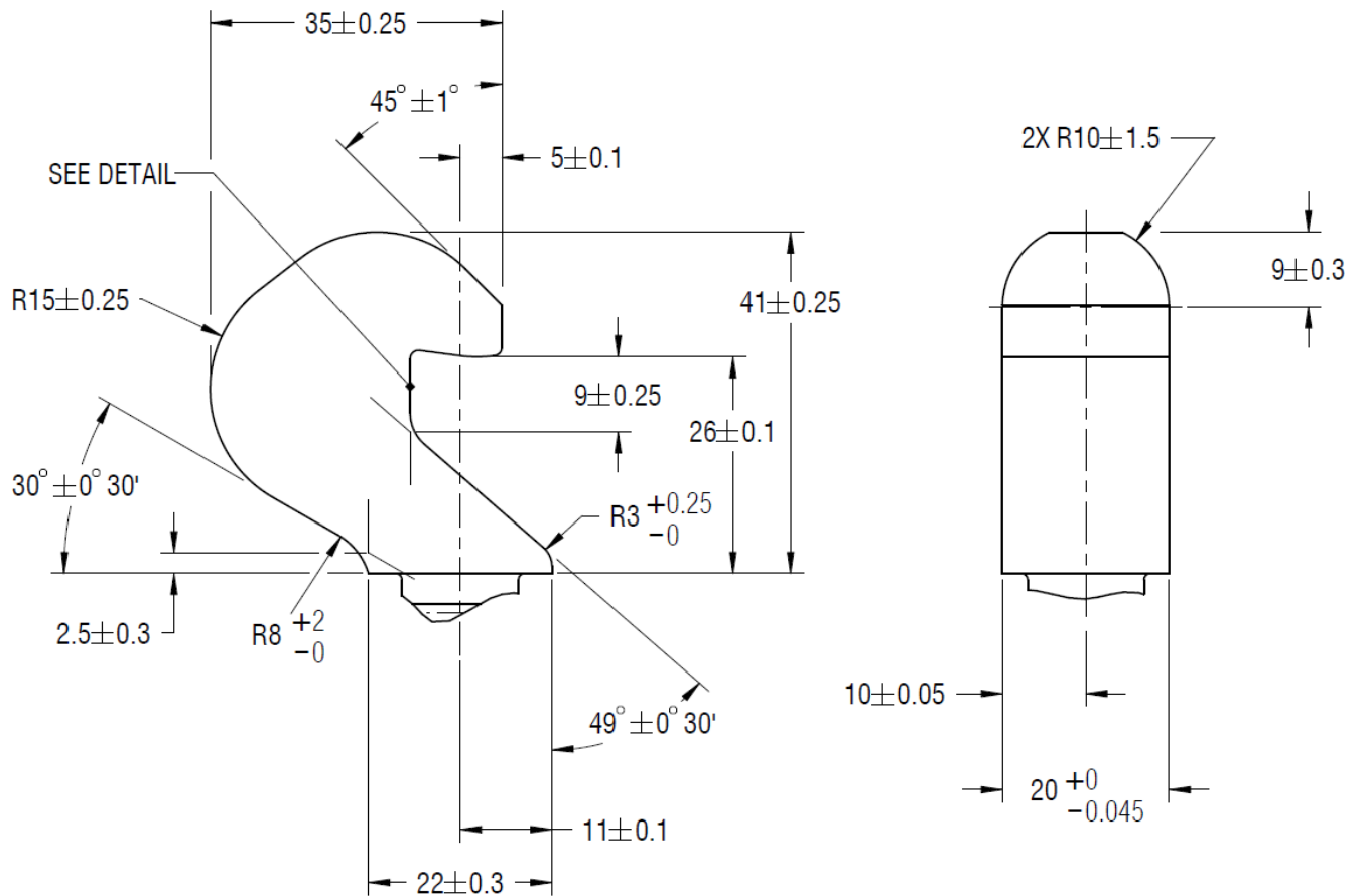
Figure 3-16a: Passive Hook
