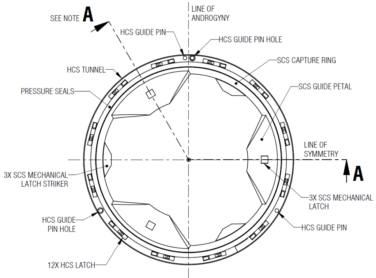
Figure 3-1: Androgynous Docking Interface – Axial View
