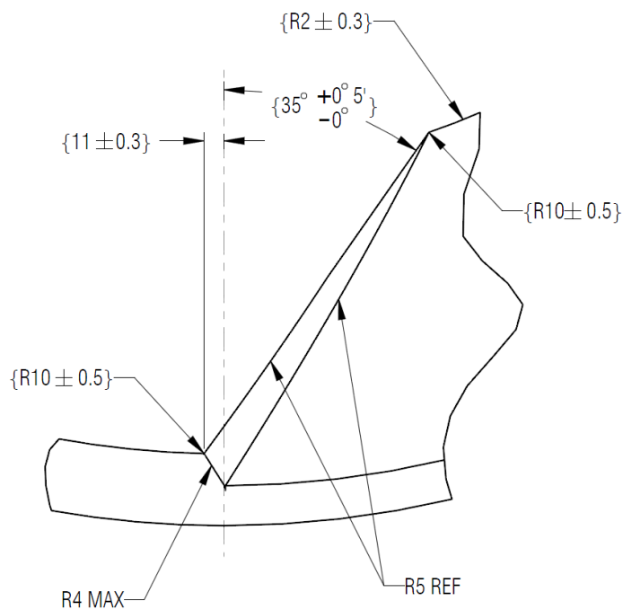
Figure 3-5b: Petal Profile Detail
