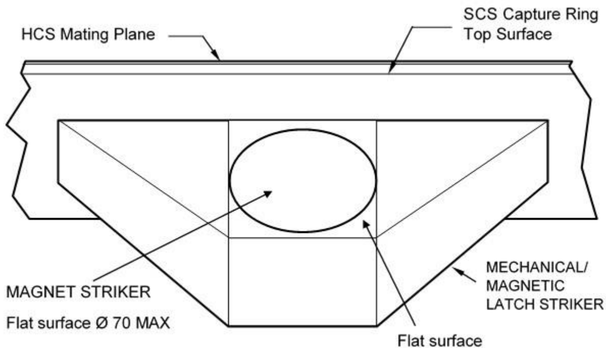
Figure B-2: Radial View
